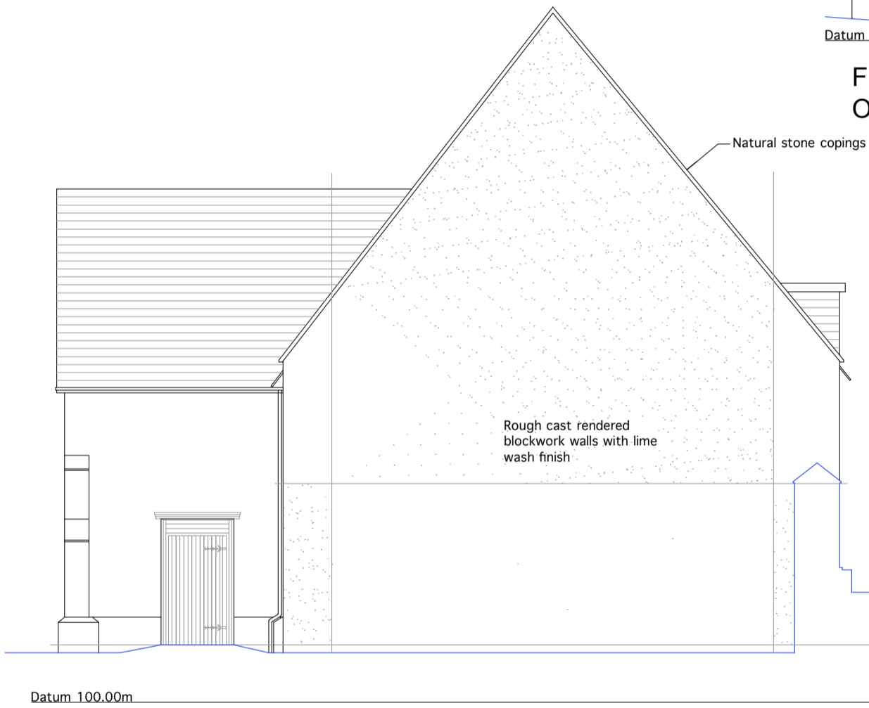
SIDE (SOUTH) ELEVATION Option 1
